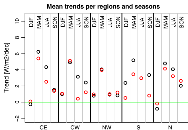
Figure 8. Trends ( \text{W/m}^2/\text{decade} ) of surface solar radiation of (black) stations and (red) SARAH-2 data, shown separately for region and season during the full time period of 1983–2015. Regions: CE = central east, CW = central west, NW = northwest, S = south, and N = north.
