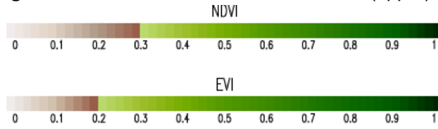
Figure 7: MODIS VI Color Palettes for NDVI (upper) and EVI (lower) products as used in this
