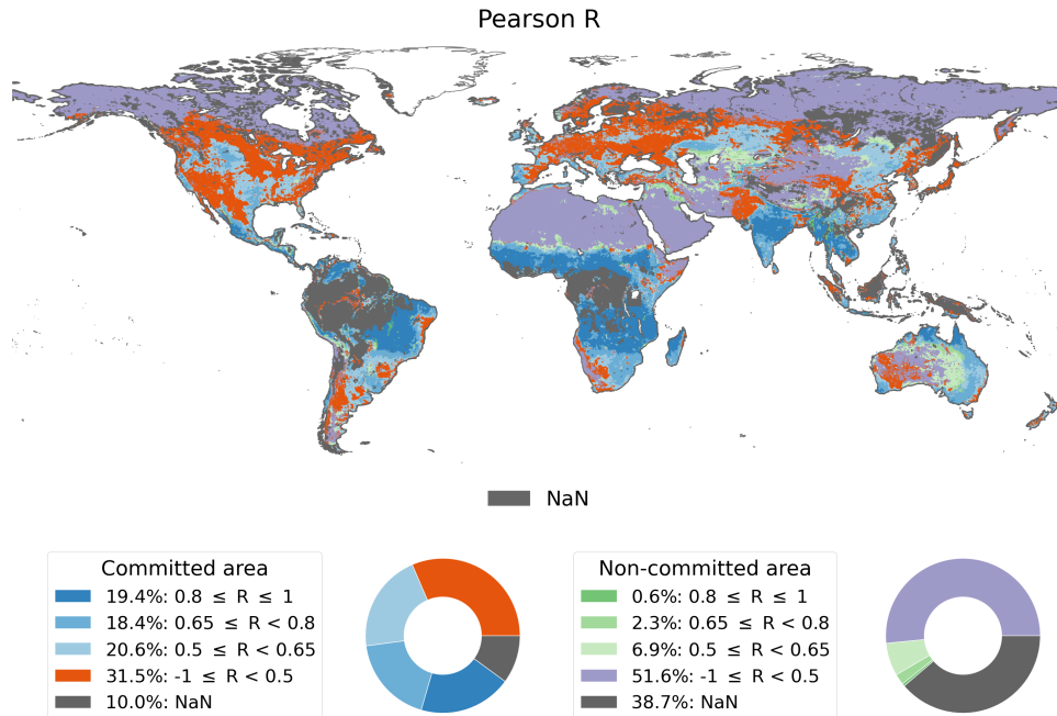
Figure 5.8: Summary of validation results of H115 SSM CDR for the period 2007-01-01 until 2018-12-31. The percentage of non-valid and valid results is split into the committed and non-committed product area. The valid results for both areas are further divided into the pre-defined thresholds. The map on top depicts the spatial distribution of the different groups.
