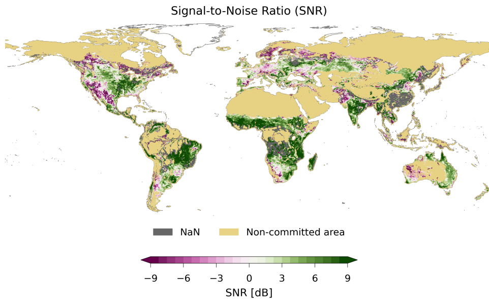
Figure 5.2: The global maps (global (a) and committed product area (b)) show the Signal-to-Noise-Ratio (SNR) expressed in dB for the H119 SSM CDR.
