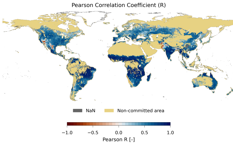
Figure 5.4: The global maps (global (a) and committed product area (b)) show the Pearson correlation coefficient for the H119 soil moisture CDR.
