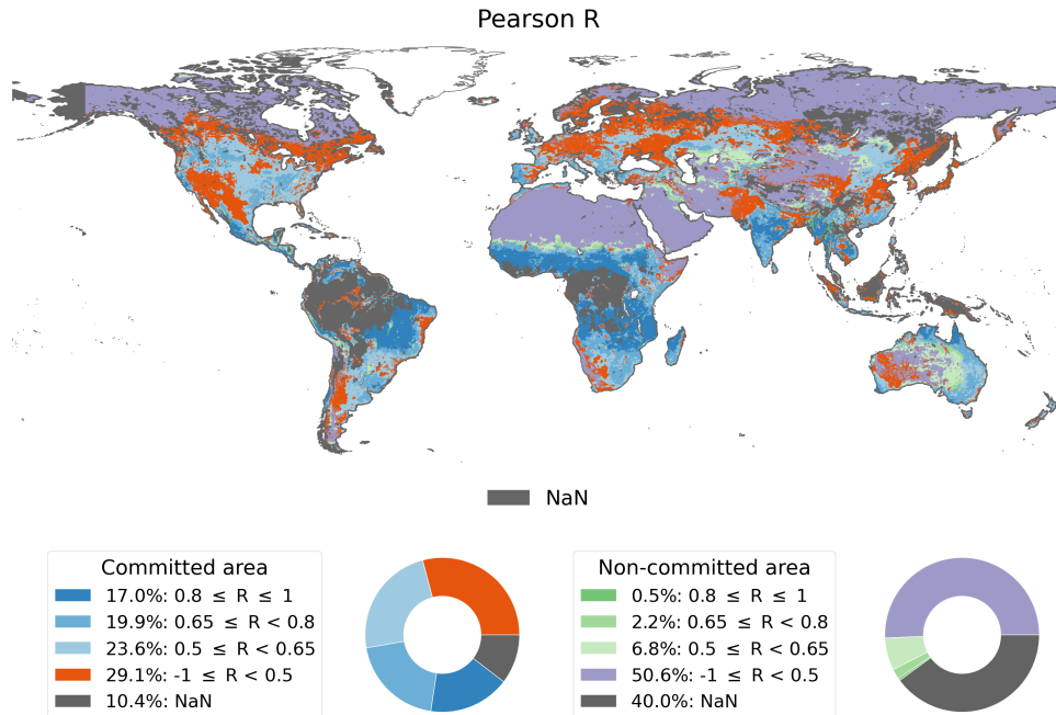
Figure 5.5: Summary of validation results of H119 CDR for the period 2007-01-01 until 2020-12-31. The percentage of non-valid and valid results is split into the committed and non-committed product area. The valid results for both areas are further divided into the pre-defined thresholds. The map on top depicts the spatial distribution of the different groups.
