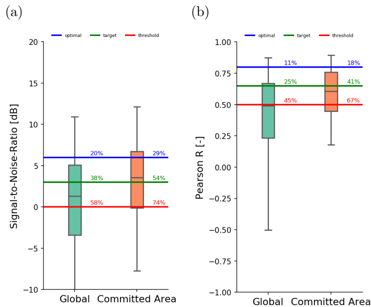
Figure 5.1: The boxplots indicate the distribution of the quality benchmarks globally and just for the committed area. A percentage of locations exceeding each of the three thresholds is indicated as well.
