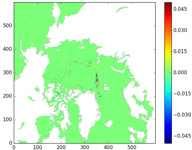
Fig. 3. Difference (unit:m) in the retrieved sea ice thicknesses between v3.2 and v3.1. Date: 2018-10-28
