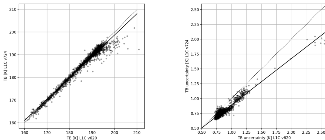
Fig. 4. Left panel: comparison between the re-gridded brightness temperatures v620 and v724 (TB unit: K). For the re-gridding, L1C sea product is used which includes about 200 km land along the coastlines. Right panel: comparison between the re-gridded brightness temperatures uncertainty v620 and v724 (TB uncertainty unit: K). Each dot represents the mean over the entire northern hemisphere grid calculated daily over the Winter seasons 2010-2020.
