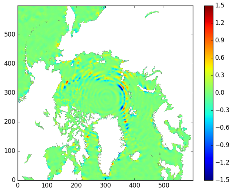
Fig. 2. Interpolated JRA55 surface temperature difference (unit: K) between v3.2 and v3.1. Date: 2018-10-27-12
