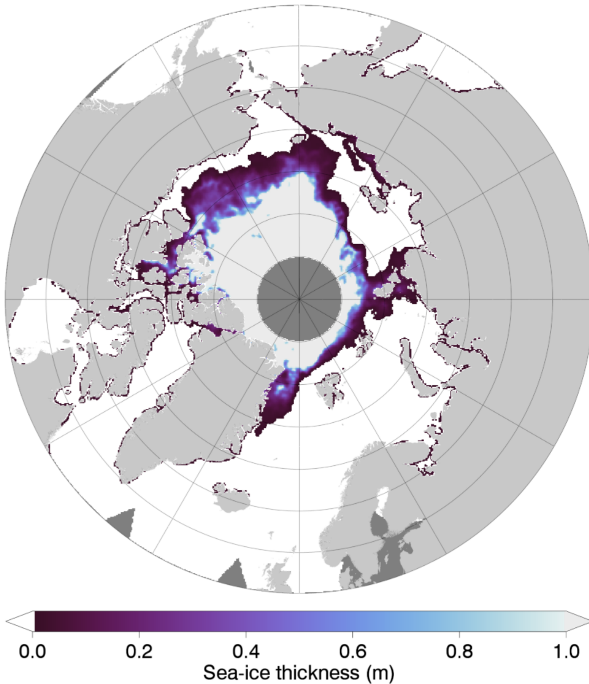
Fig. 1. Sea ice thickness map in the Arctic, 2021.10.12
