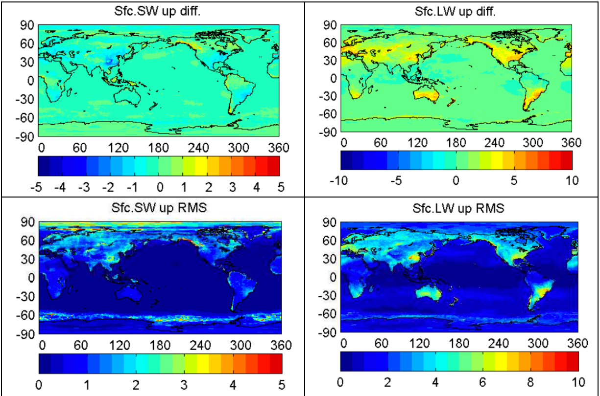
Figure 2. (top) Monthly mean difference and (bottom) RMS difference between cloud-removed and clear-sky fraction-weighted (left) surface upward shortwave fluxes and (right) surface upward longwave fluxes in W m^{-2} . The mean difference and RMS difference are computed using 10 years of monthly mean 1^{\circ} \times 1^{\circ} gridded fluxes from March 2000 through February 2010. The mean difference is defined as the cloud-removed minus clear-sky fraction-weighted fluxes.
