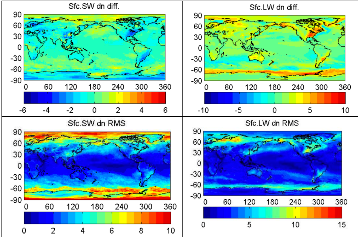
Figure 1. (top) Monthly mean difference and (bottom) RMS difference between cloud-removed and clear-sky fraction-weighted (left) surface downward shortwave fluxes and (right) surface downward longwave fluxes in \text{W m}^{-2} . The mean difference and RMS difference are computed using 10 years of monthly mean 1^\circ \times 1^\circ gridded fluxes from March 2000 through February 2010. The mean difference is defined as the clouds-removed minus clear-sky fraction-weighted fluxes.
