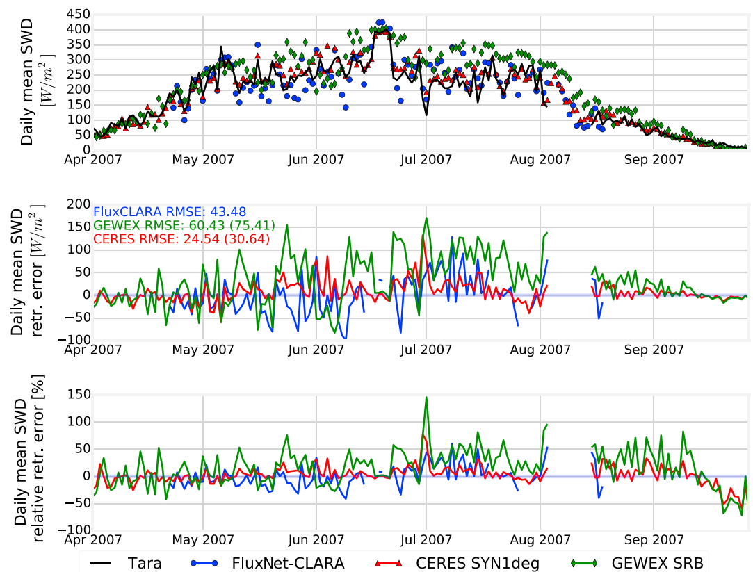
Figure 4. Validation of daily mean SWD flux estimates from CERES SYN1deg, GEWEX SRB, and FluxNet-CLARA against in situ SWD observations made at Tara ice camp during polar summer 2007. The RMSE in parentheses is for a subset corresponding to the FluxNet-CLARA temporal coverage. (top) Retrieved and measured daily mean fluxes. (middle) Satellite-based retrieval errors versus in situ. (bottom) Relative retrieval errors.
