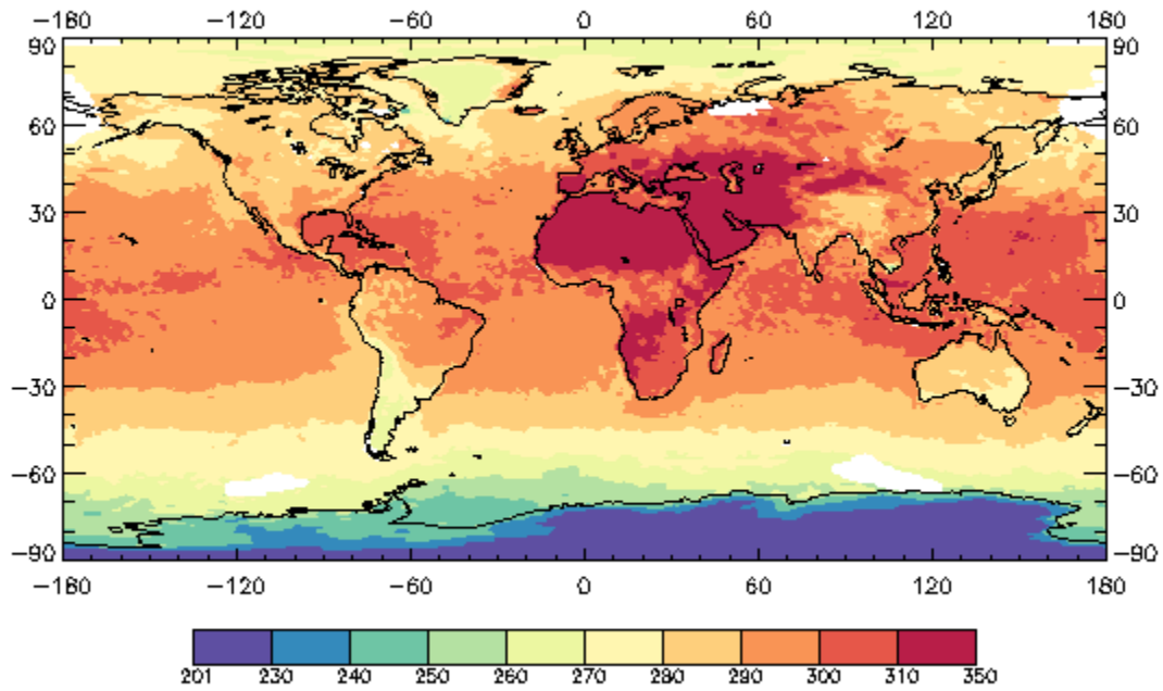
HGG Clear Sky Temperature (K), July 2007 Day 15 UTC 1200
