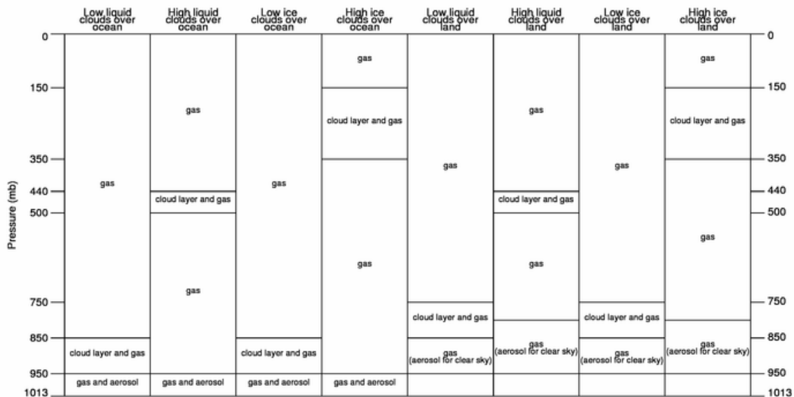
Figure 7: Schematic of atmospheric layers in VIS RTM
