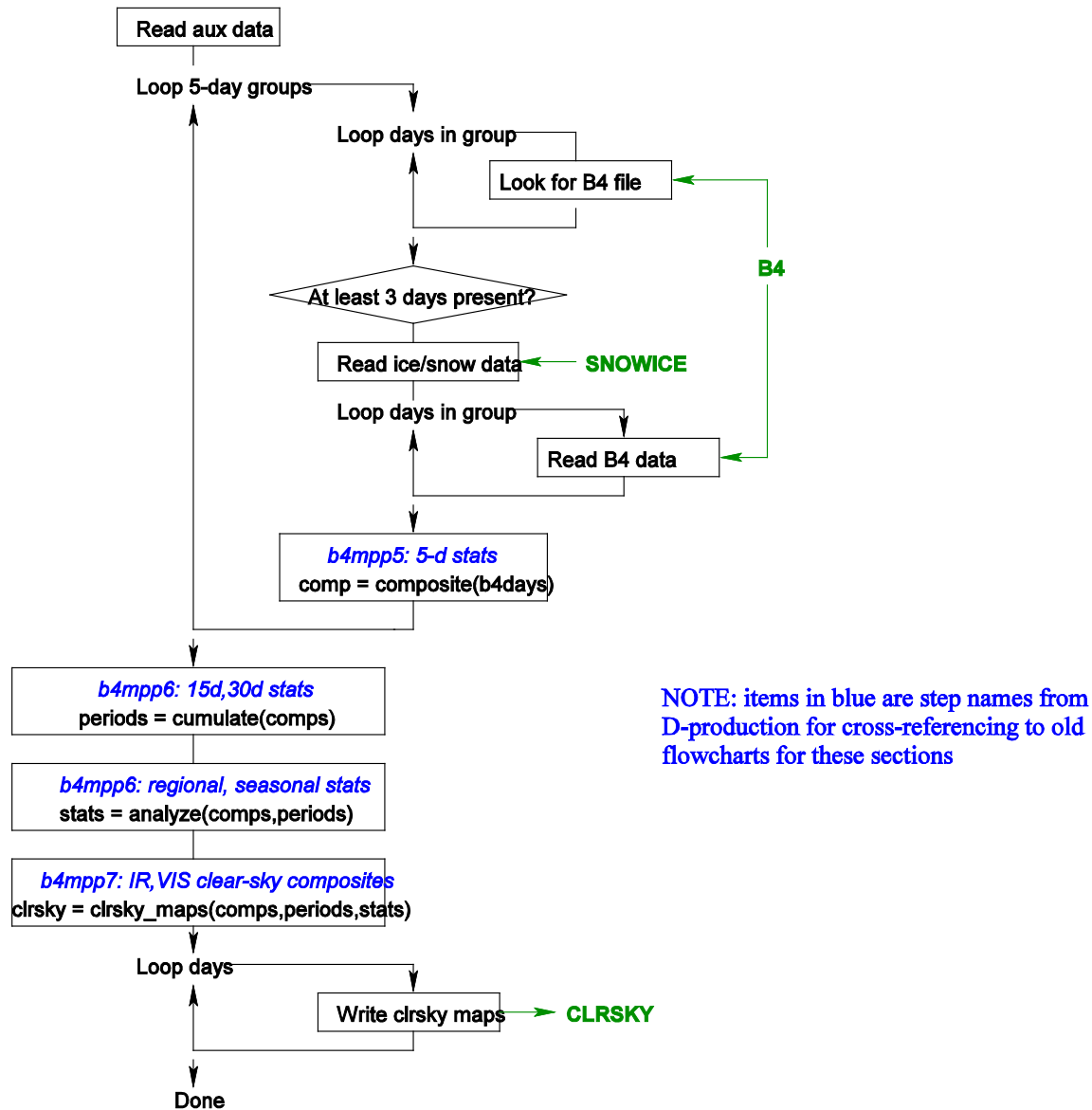
Figure 12: CLRSKY main program
