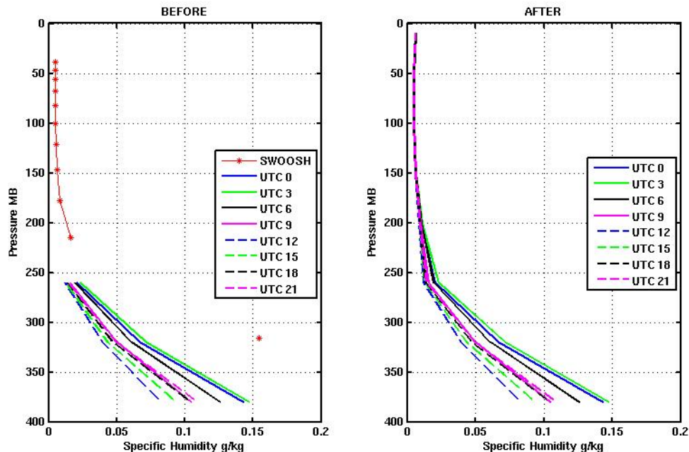
Figure D.1.3 Example of reconciliation of HIRS and SWOOSH vertical humidity profiles
