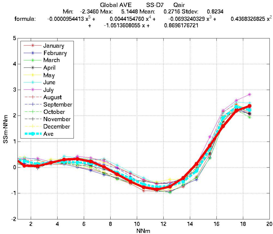
FIGURE D.1.2. Annual Mean QA difference between NNHIRS and SeaFlux as a function of NNHIRS QA
