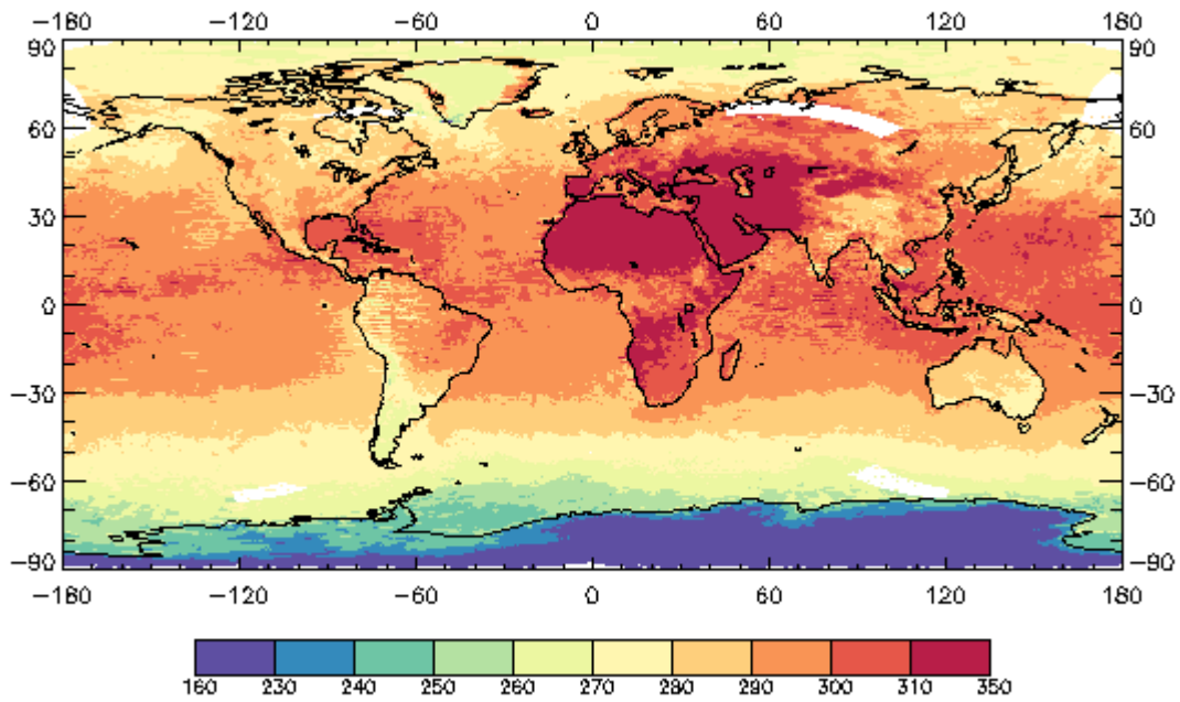
HXG Clear Sky Temperature (K), July 2007 Day 15 UTC 1200
