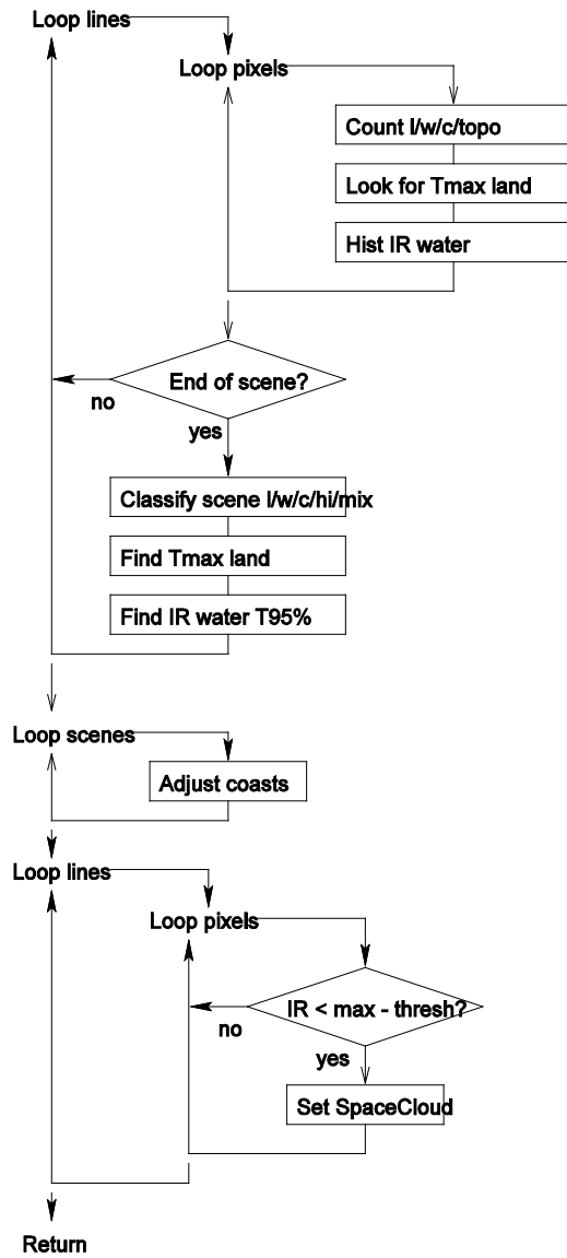
Figure 10: B4PROD subroutines time_test and classify
