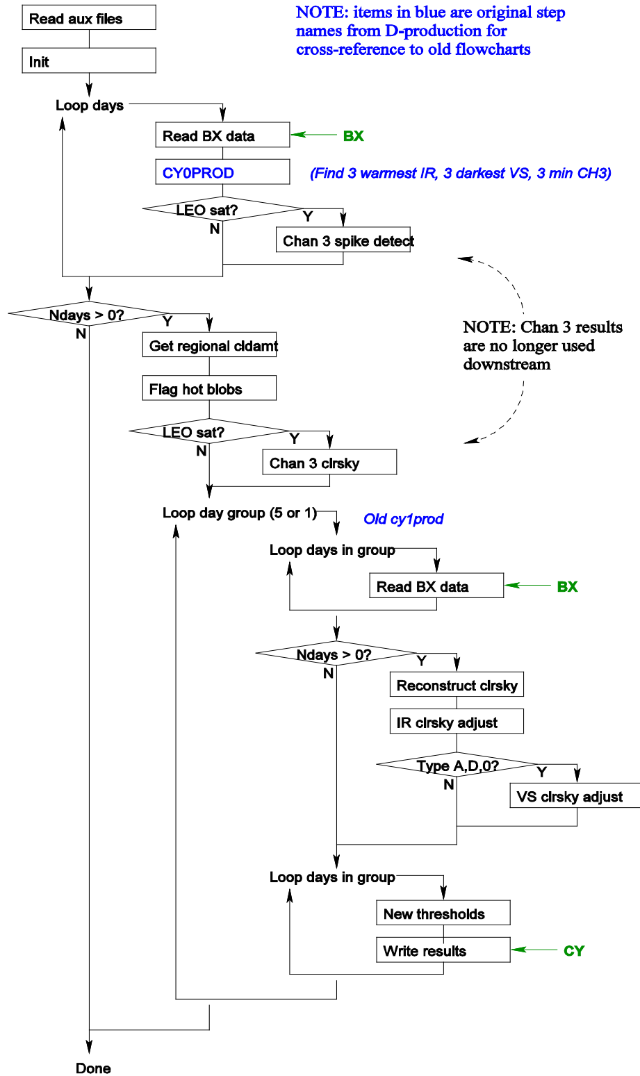
Figure 17: CYPROD Main Program
