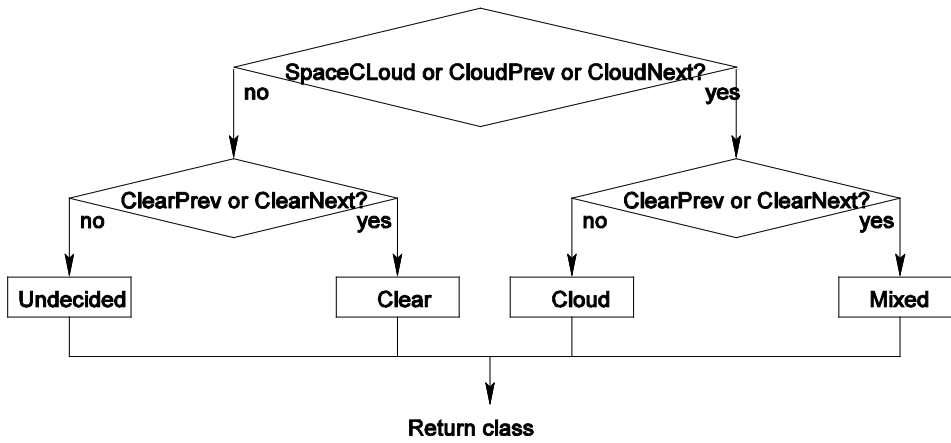
Figure 11: B4PROD subroutines time_test and classify
