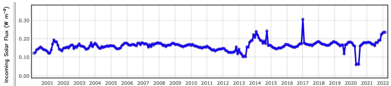
Figure 1. The EBAF Ed4.2 minus Ed4.1 total solar incoming difference.
